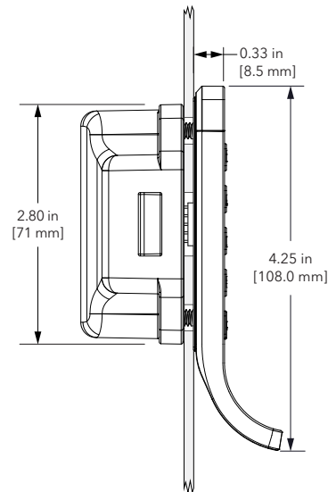
Side View-Pin Connector
