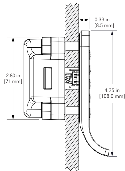
Side View-Cable
