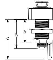
Lifter Cam
