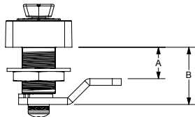
Offset Cam
