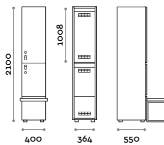
VANB35-23 Singola colonna 2 ante per panca Single column 2-tiers locker, bench version
