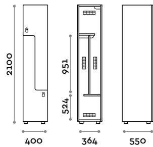
TANB39-23 Singola colonna 2 ante a "L" Single column locker, 2 L-shaped doors
