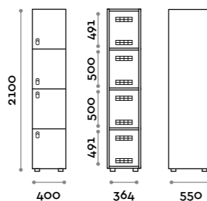
TANB324-23 Singola colonna 4 ante Single column 4-tiers locker
