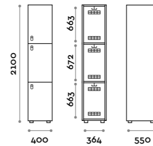
ANB323-23 Singola colonna 3 ante Single column 3-tiers locker
